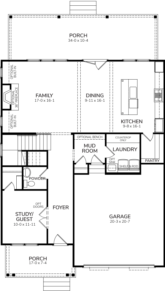
First Floor
