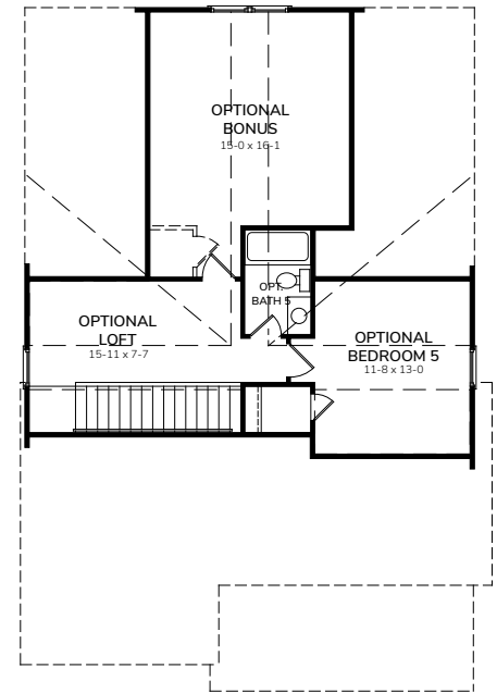
Third Floor Opt 3rd Floor
