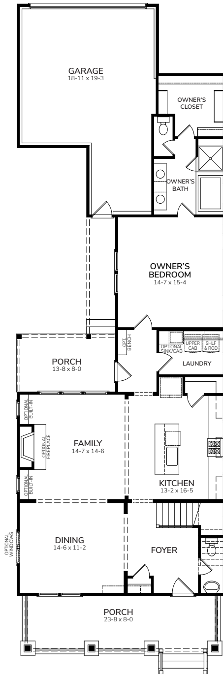
First Floor
