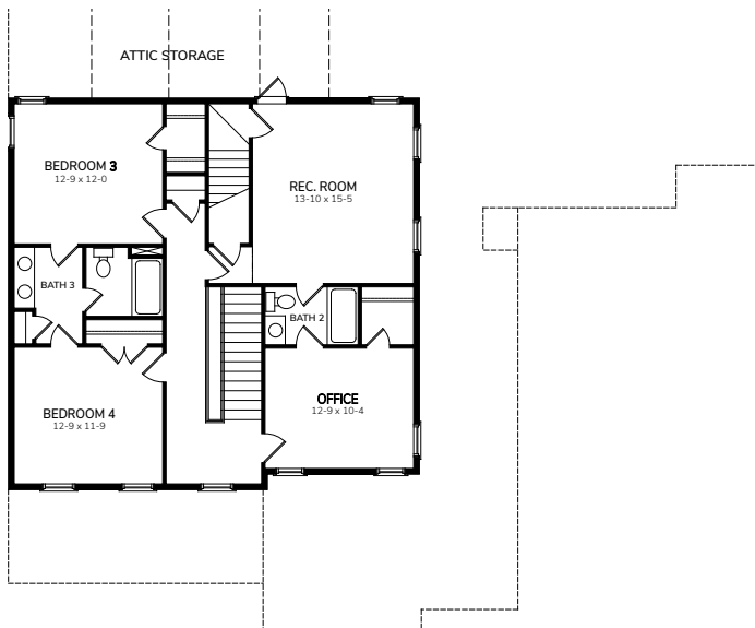
Opt Second Floor with Attic
