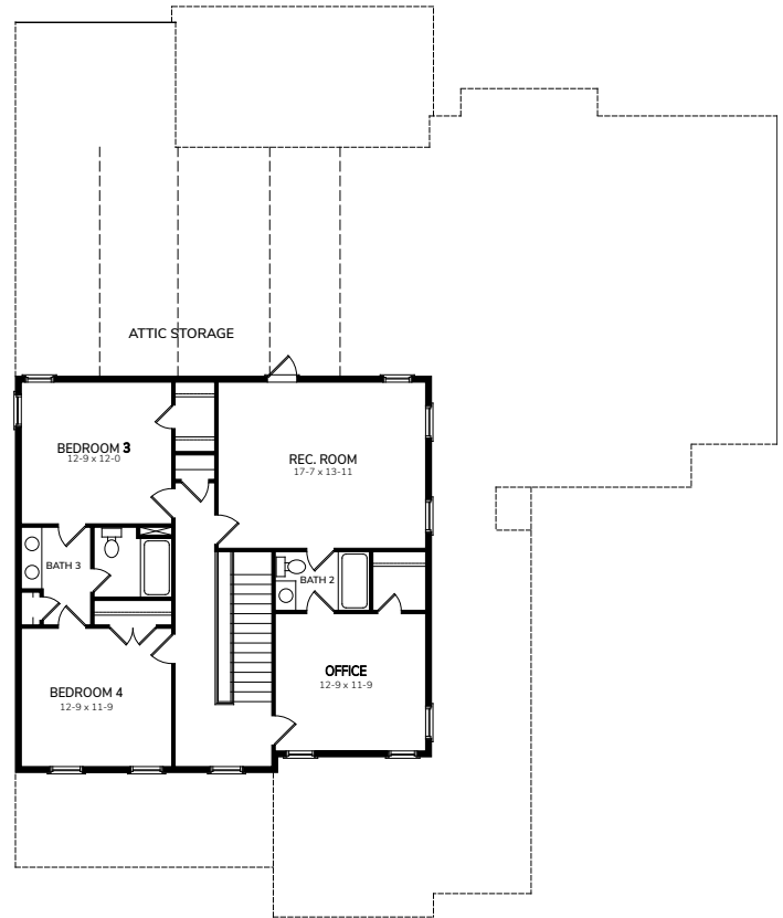
Second Floor
